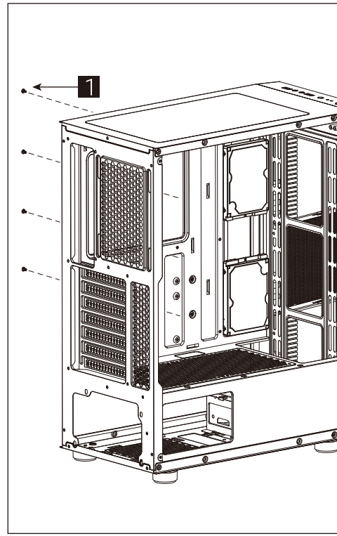
(5b) Install 2.5" SSD x 2
