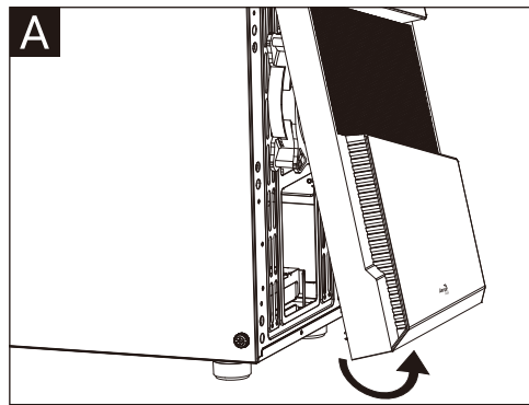
(6a) Install Front Radiator x 1
