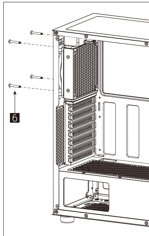
(6b) Install Rear Radiator x 1
